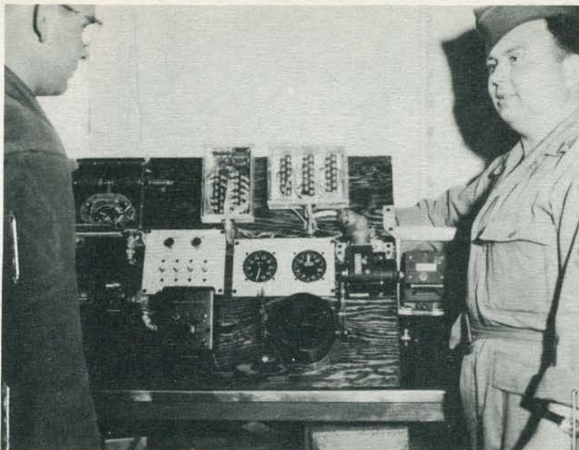
M/Sgt. Charles J. Jones made this visible mock-up electron supercharger regulator. This mock-up tested instruments which did not function properly. All the moving parts of the instrument being checked could be observed through Plexiglas.
