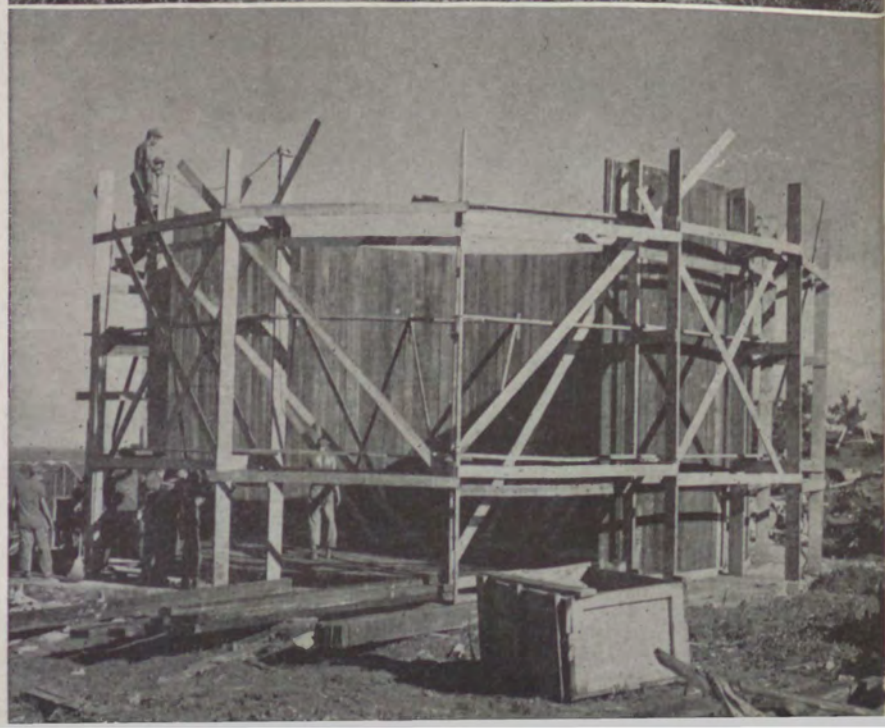
Construction of a 126,000-Gallon Water Tank
